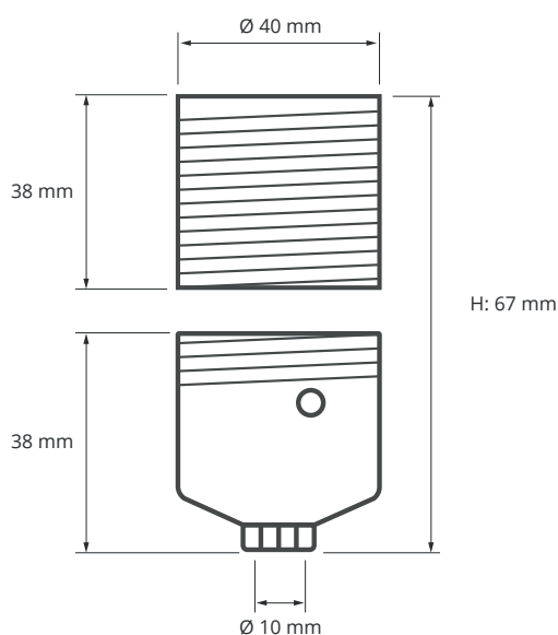
Frame top & bottom part - H = Screwed together height
