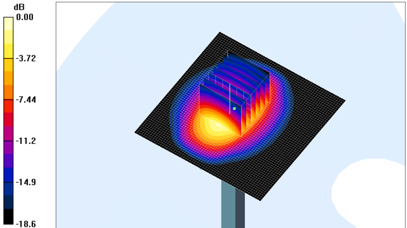
Fig. 12: 1950 MHz validation result
