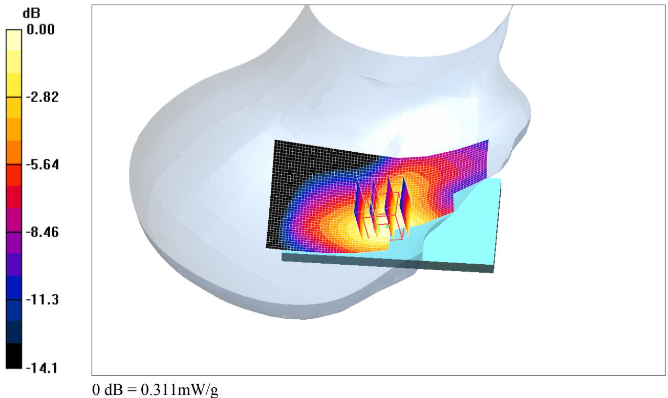
Fig. 6: SAR distribution for WCDMA2100 of the mobile phone alone: channel 9750 (1950.0 MHz), cheek position, right side
