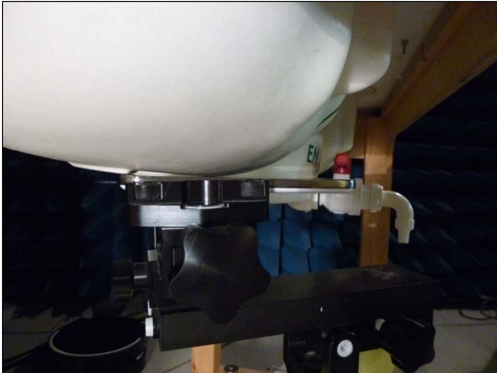
Fig. 8: Mobile phone in cheek position on right side
